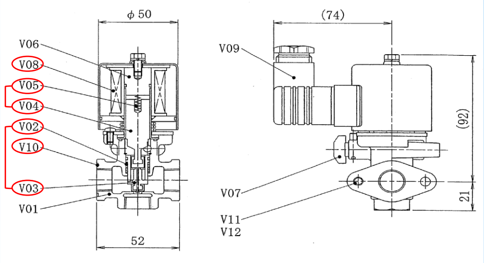
SOLENOID VALVE SV1, SV2, SV3, SV9
