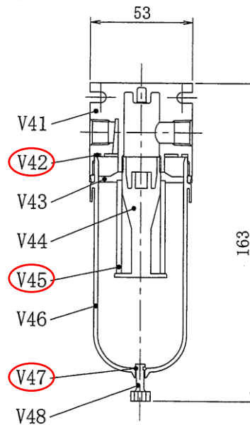
AIR FILTER (AF1)
