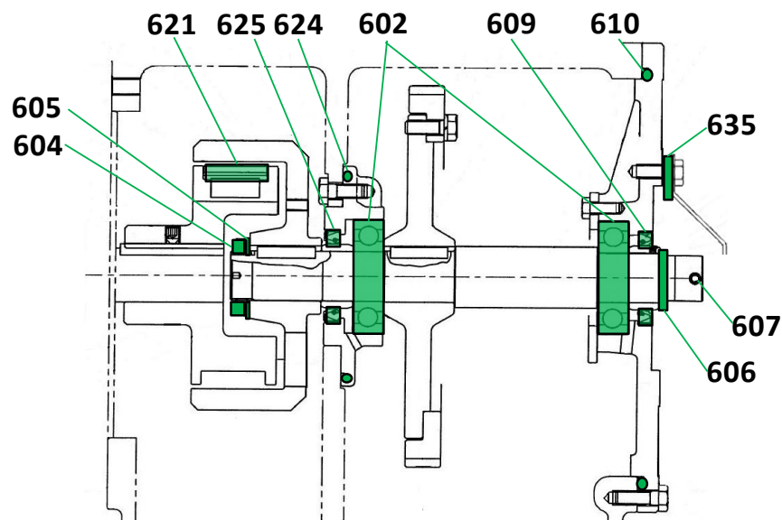
Horizontal Shaft assy
