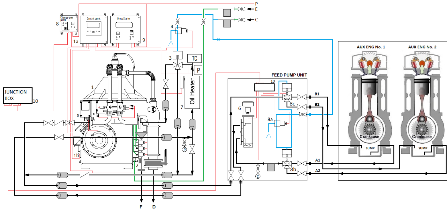
1.5 CHANGE-OVER SYSTEM IN CASE OF ENGINE No. 2
