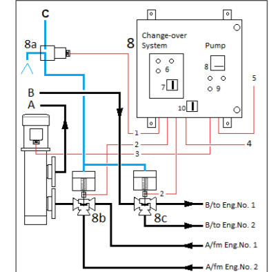
1.5 CHANGE-OVER SYSTEM IN CASE OF ENGINE No. 2
